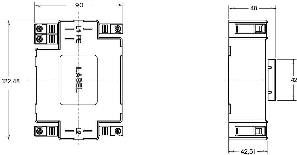
IQ-LCF-040-1P Power Line Filter
