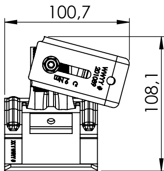
Transport position
