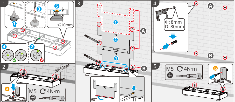
Installation of battery, inverter & battery protective cover. / 安装电池、逆变器和电池防护罩
