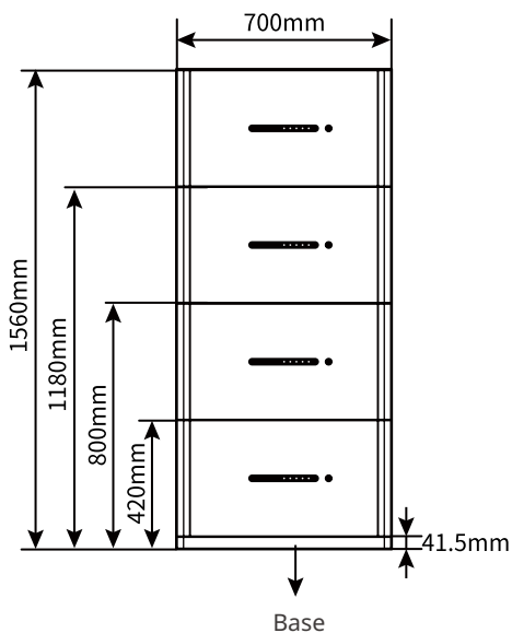
Battery group dimensions (ground installation)
