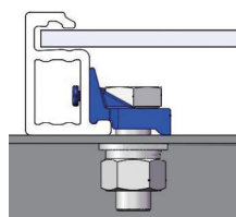
Installation with Mounting Hole Holder:
