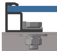
Installation with Mounting Hole Bolts:
