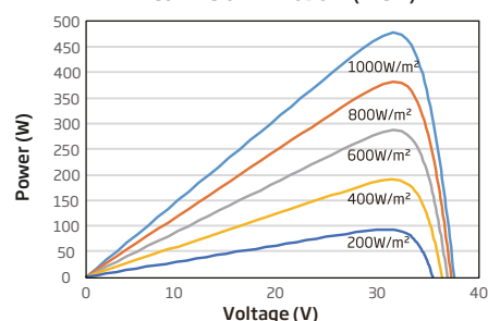
P-V CURVES OF PV MODULE (475W)
